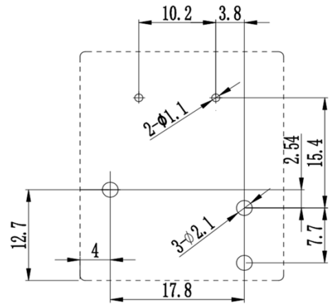
Bottom View Layout
