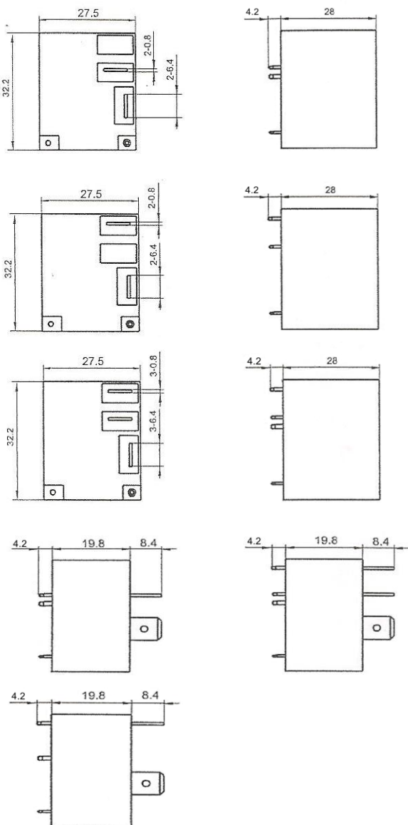
Outline Dimension
