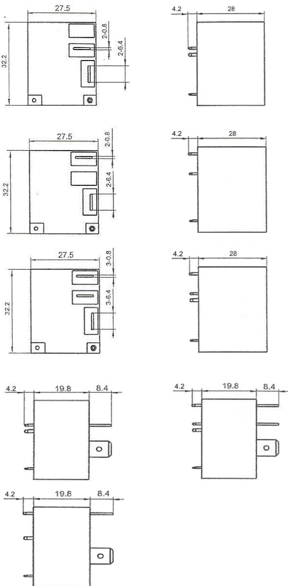
Outline Dimension
