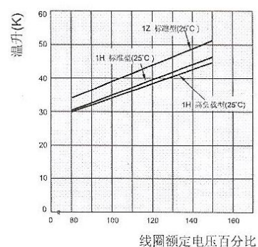
Temperature Rising
