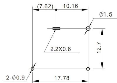
Bottom View Layout
