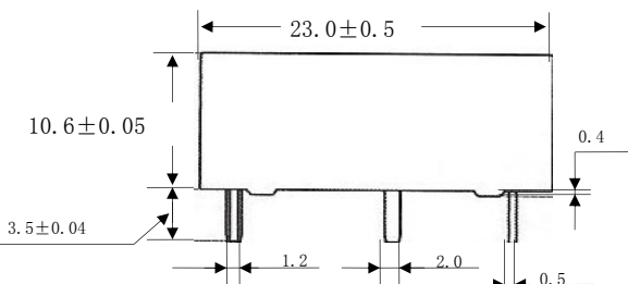
Outline Dimension(1)
