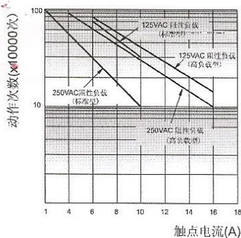
Electric endurance curve
