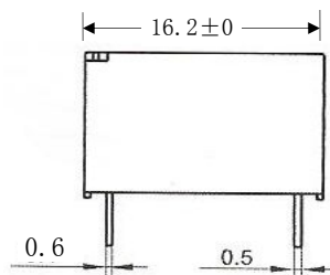
Outline Dimension(2)
