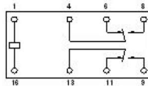
Bottom View Layout
