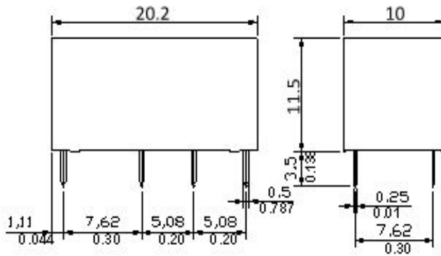
Outline Dimension
