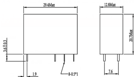
Outline Dimensions
