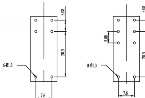
Bottom View Layout
