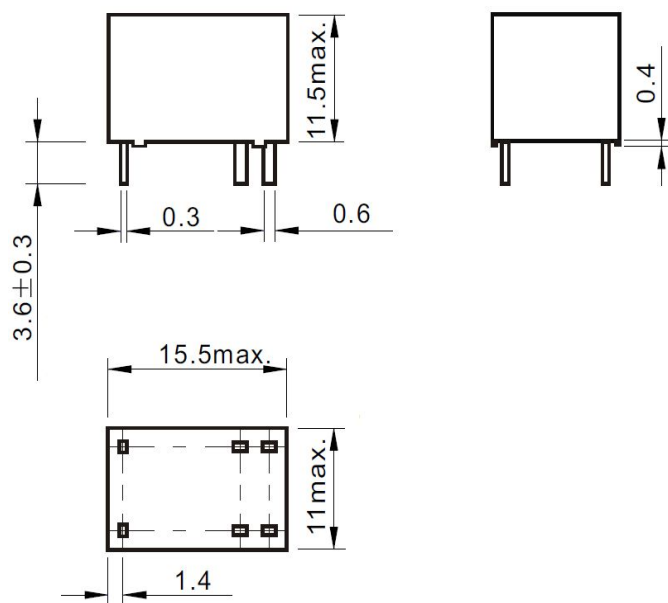
Outline Dimension
