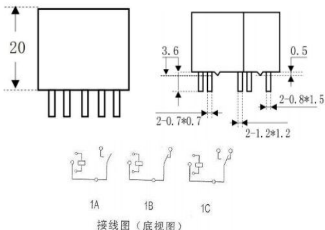
Wiring Diagram (Bottom View)
