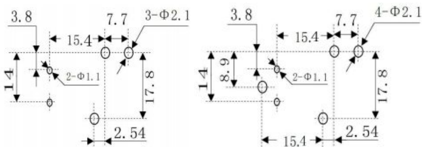
Bottom View Layout
